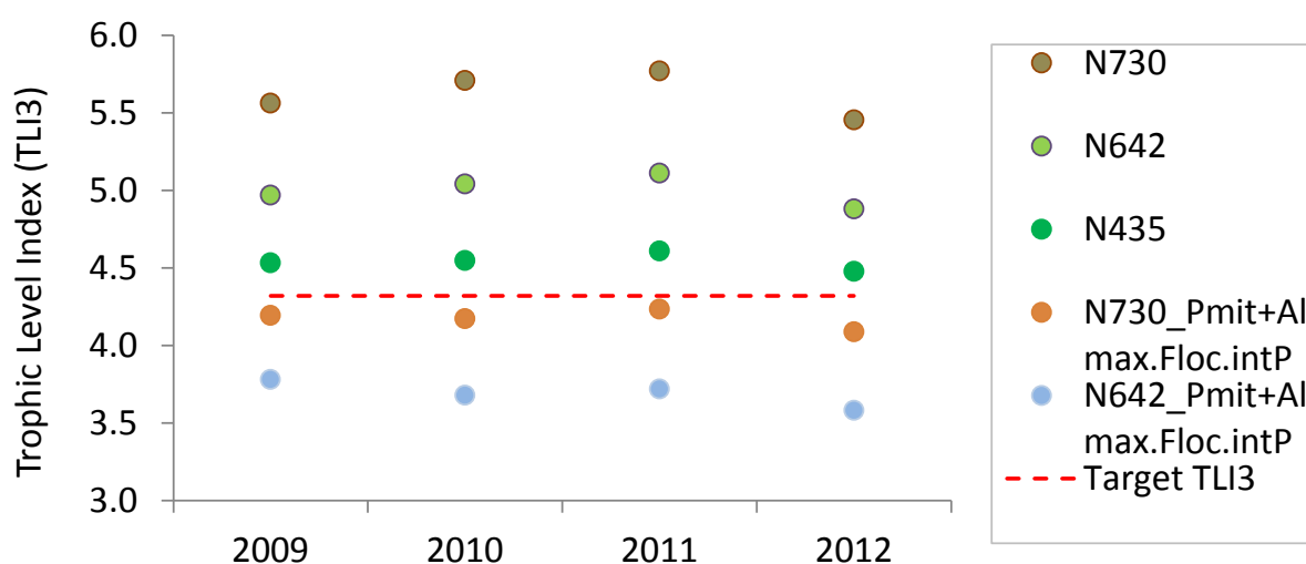
Figure 26. Yearly TLI values for scenario simulations. Refer to Table 2 for an explanation of each scenario name. The dashed red line is the TLI3-adjusted target for Lake Rotorua (TLI3 = 4.32).
