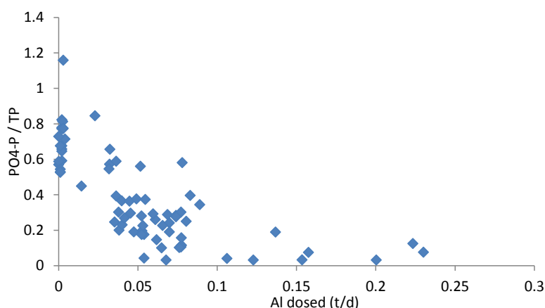
Figure 17. Relationship between daily aluminium dose and observed ratio of DRP to TP downstream of the dosing location in Uthina Stream. Data provided by Alastair McCormack and Paul Scholes, Bay of Plenty Regional Council.
