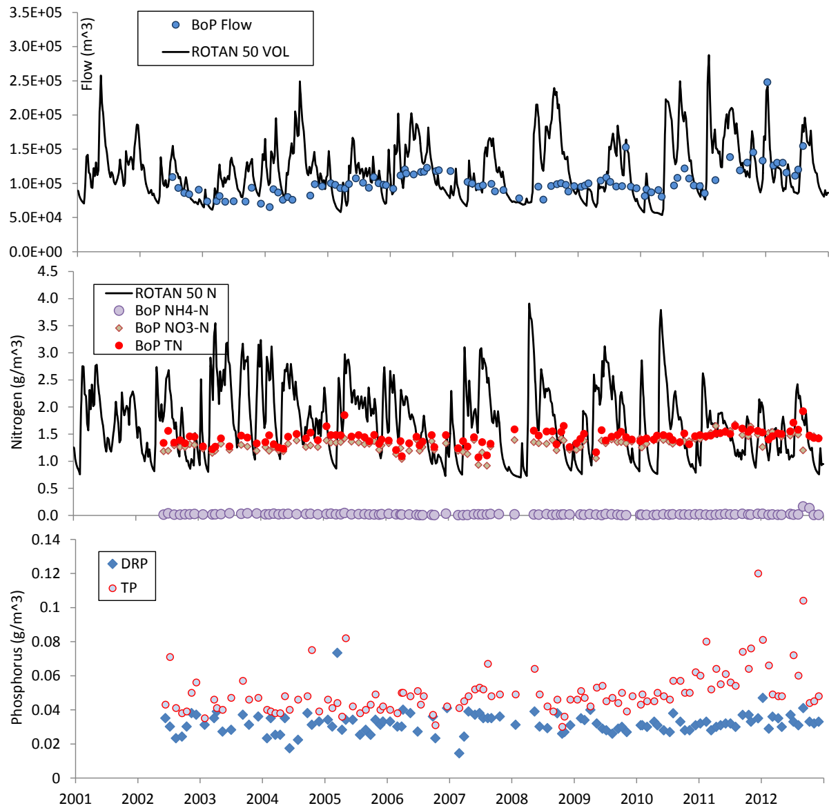
Figure 13. Time-series plots of Bay of Plenty inflow monitoring data (dots) and ROTAN output (lines) for the Waiteti stream sub-catchment, for A) daily flow, B) nitrogen, and C) phosphorus.
