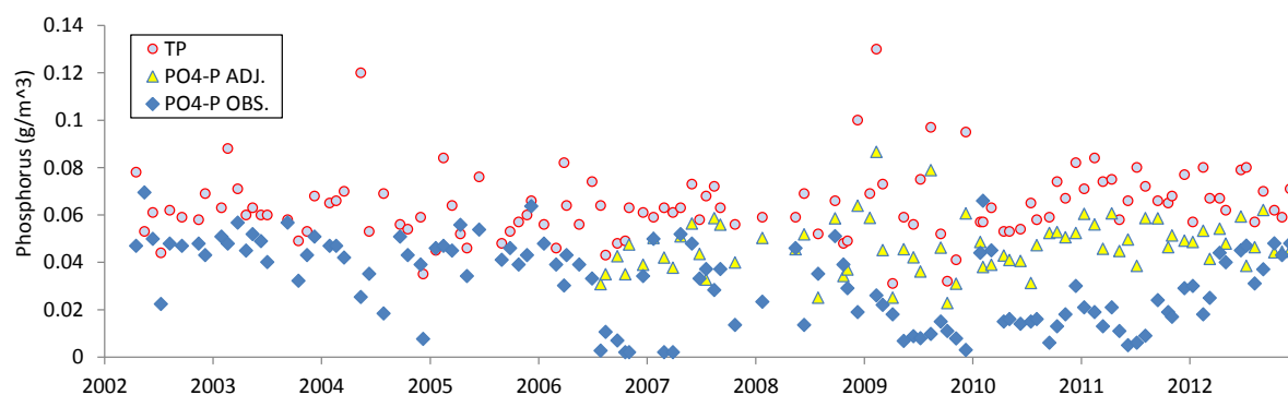
Figure 18. Time-series of inflow measurements in the Uthina inflow for TP (red dots), DRP (blue diamonds). Green triangles represent estimated DRP if alum dosing had not been undertaken 2006 – 2012. This was estimated using an average of DRP:TP for each month of the period before alum dosing commenced.
