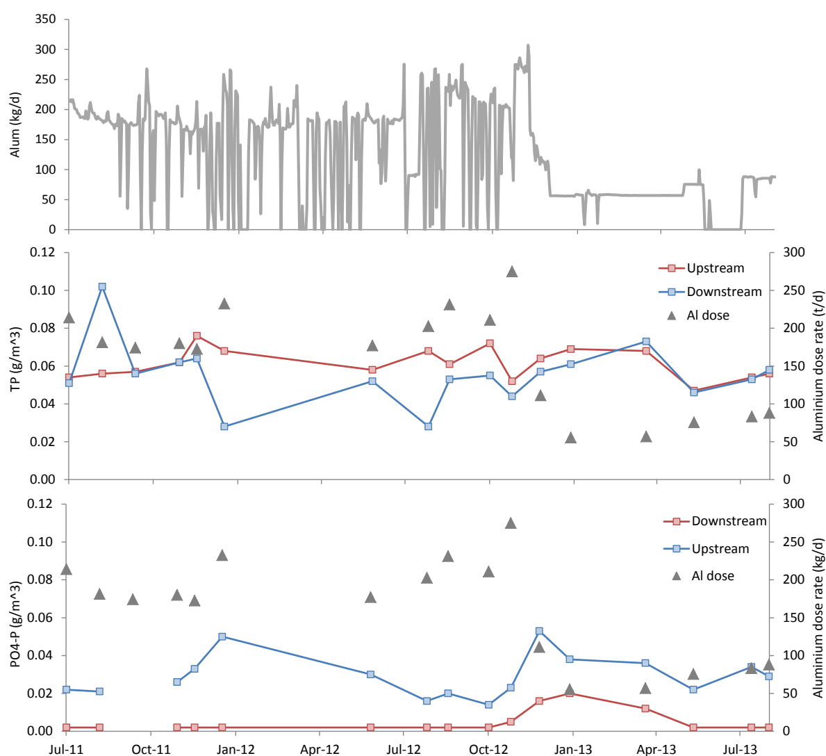
Figure 19. A) Dose rate of aluminium to the Puarenga inflow (assuming 4.2% of alum product is aluminium), B) Upstream and downstream TP concentrations with corresponding Al dose rate for spot measurements 2011 – 2013, C) Upstream and downstream DRP concentrations with corresponding Al dose rate for spot measurements 2011 – 2013. Data provided by John McIntosh and Bay of Plenty Regional Council.
