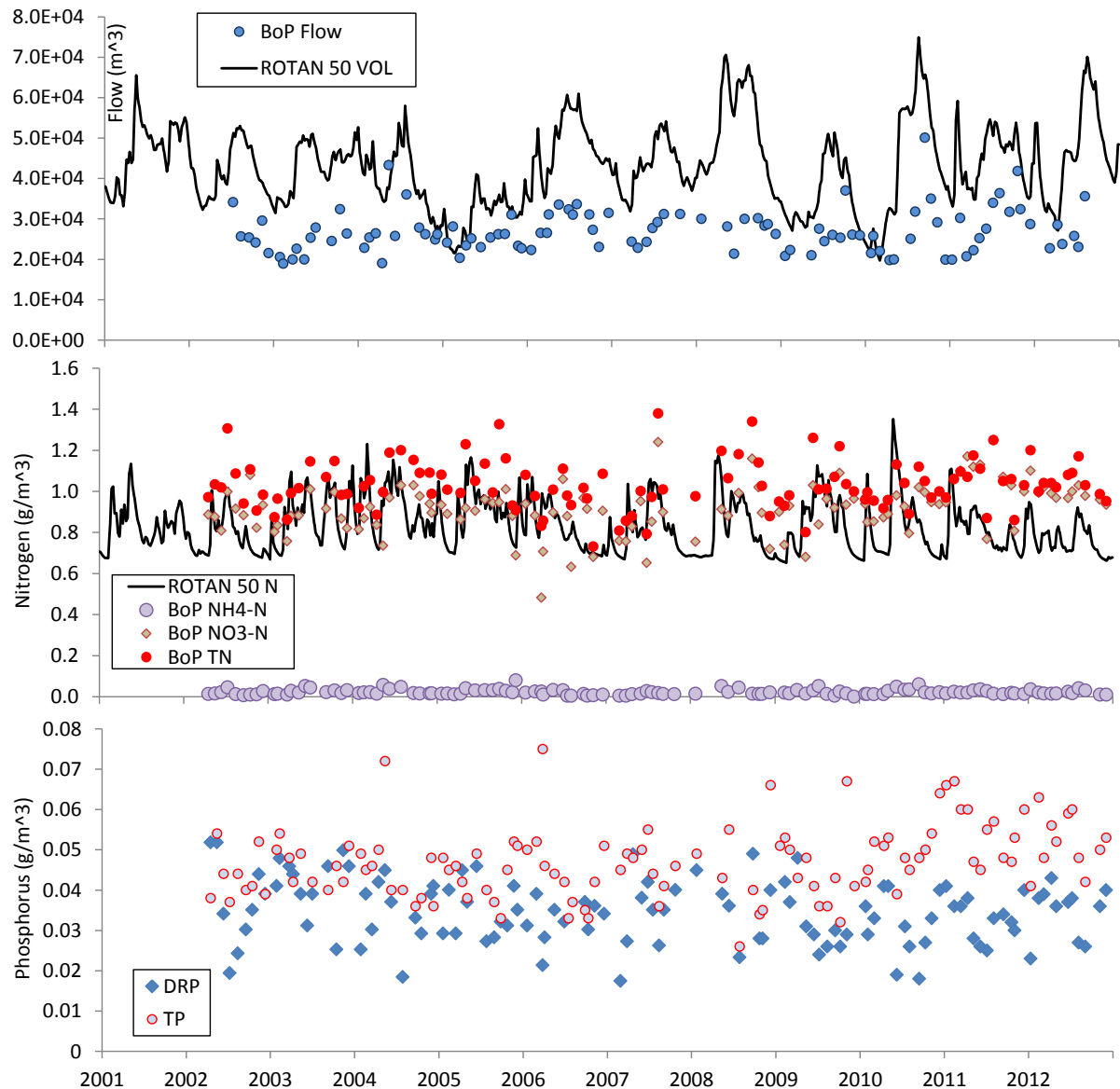
Figure 12. Time-series plots of Bay of Plenty inflow monitoring data (dots) and ROTAN output (lines) for the Waiowhiro stream sub-catchment, for A) daily flow, B) nitrogen, and C) phosphorus.
