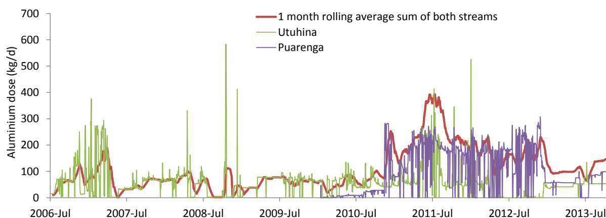
Figure 15: Alum dosing in Utuhina (green line) and Puarenga Streams (purple line), and combined dosing (1 month rolling average; red line). Data supplied by Alastair McCormack, Bay of Plenty Regional Council.
