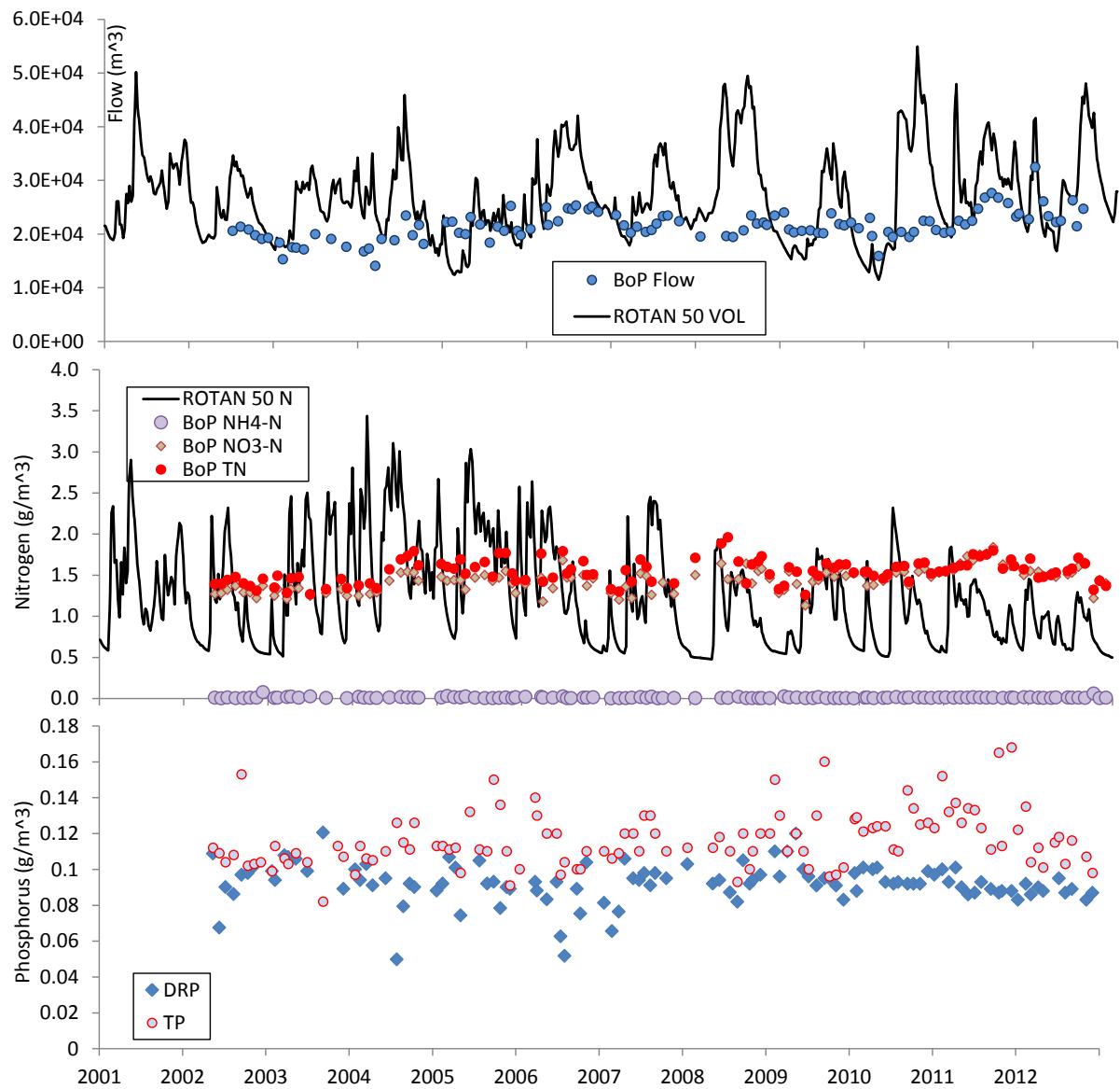
Figure 10. Time-series plots of Bay of Plenty inflow monitoring data (dots) and ROTAN output (lines) for the Waingaehe stream sub-catchment, for A) daily flow, B) nitrogen, and C) phosphorus.
