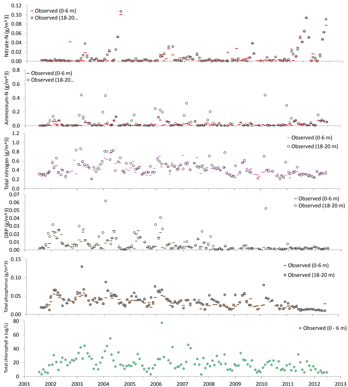
Figure 21: In-lake measurements for nitrate, ammonium, total nitrogen, dissolved reactive phosphorus (DRP), and total phosphorus at the surface (0 - 6 m) and bottom (18 – 20 m), and total chlorophyll a at the surface (0-6 m) from 2001 to 2013.
