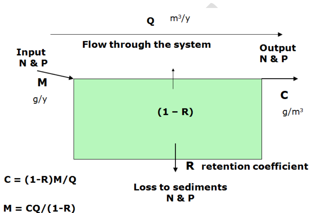
Figure 1 Schematic of lake model.
