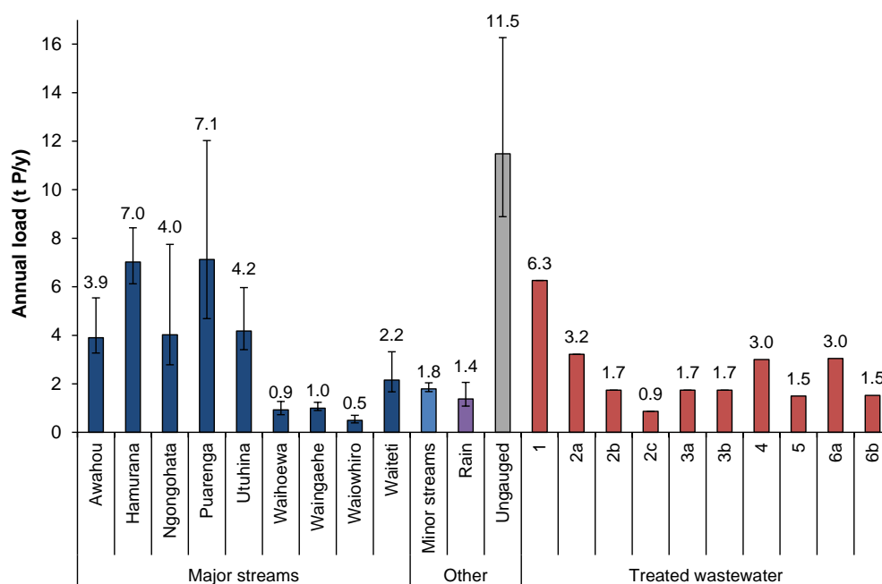
Figure 22 Summary of mean external phosphorus loads used as forcing data in baseline model simulations. Puarenga Stream loads do not reflect attenuation by alum. Vertical lines denote between-year variations.
