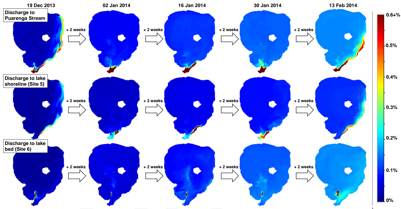
Figure 35 Comparison of simulated water column average tracer concentrations for scenarios of discharge to the Puarenga Stream, Lake Rotorua shoreline (Site 5) and the lake bed (Site 6; Map 2) during summer 2013/2014. Plots are at two-week intervals, commencing two-weeks after the simulation started.
