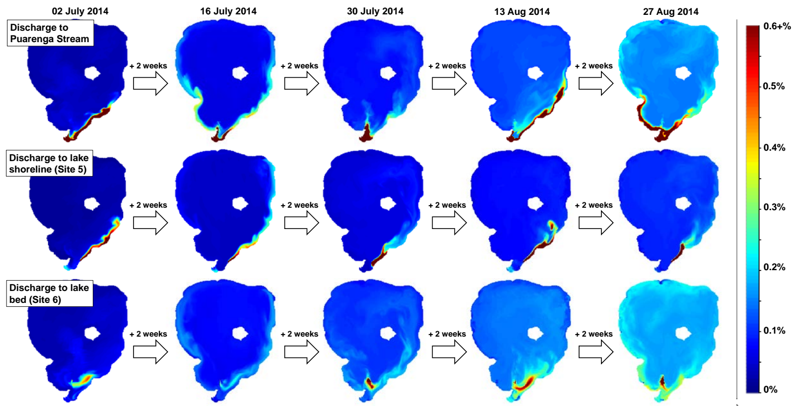
Figure 37 Comparison of simulated water column average tracer concentrations for scenarios of discharge to the Puarenga Stream, Lake Rotorua shoreline (Site 5) and the lake bed (Site 6; Map 2) during winter 2014. Plots are at two-week intervals, commencing two-weeks after the simulation started.
