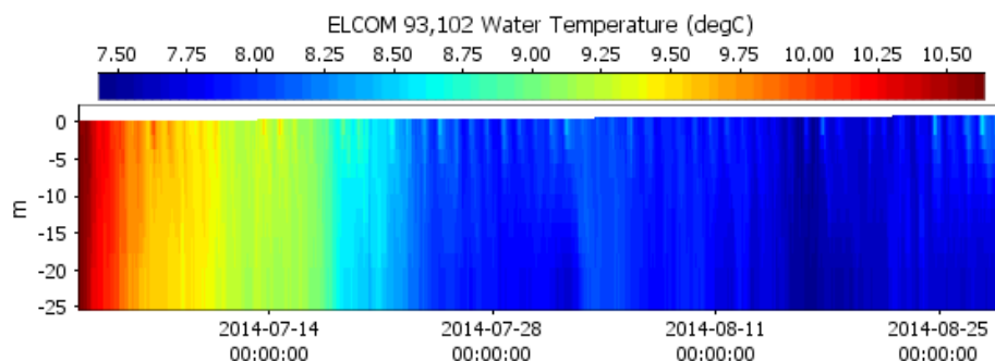
Figure 28 Simulated water temperatures during the winter (2014) modelling period.
