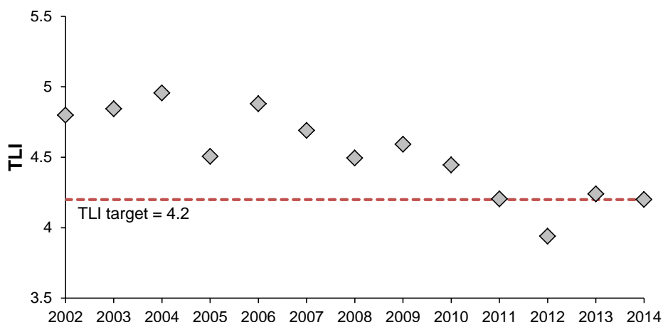
Figure 1 Annual Trophic Level Index of Lake Rotorua. Data for 2002–2012 are based on surface water samples only and thus values may differ slightly from by those used for BoPRC monitoring. Sources: 2002–2012 data (Abell et al. 2012); 2013 datum (Rotorua Te Arawa Lakes Programme 2014); 2014 datum ( http://www.rotorualakes.co.nz/lake_rotorua_facts , accessed 29 May 2015).
