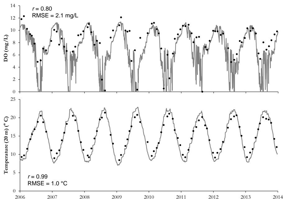
Figure 18 Comparisons of measured (circles) and modelled (line) concentrations of dissolved oxygen (DO) and temperature in bottom waters (depth = 20 m).
