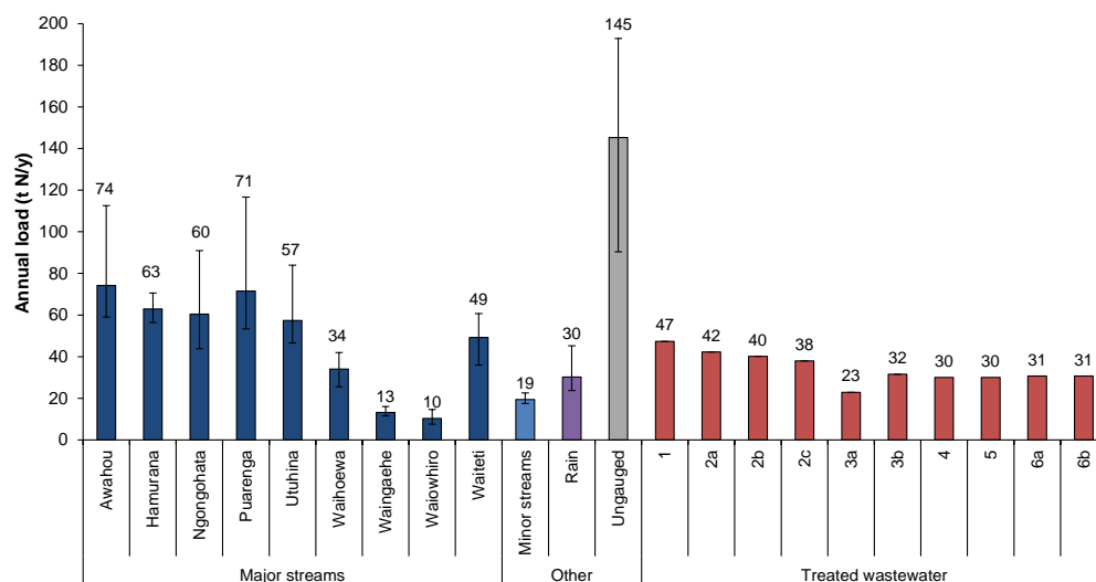
Figure 23 Summary of mean external nitrogen loads used as forcing data in baseline model simulations. Vertical lines denote between-year variations.
