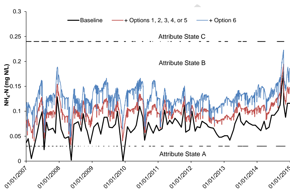
Figure 13 Estimated mean daily ammonium nitrogen concentrations in the Puarenga Stream for baseline conditions and following addition of treated wastewater. Dashed lines denote annual median values that correspond to Attribute States defined in the National Policy Statement for Freshwater Management 2014.
