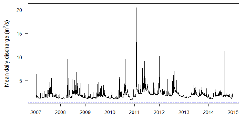
Figure 2 Puarenga Stream mean daily discharge, 2007–2014. The dashed blue line denotes the mean discharge of treated wastewater for reference.
