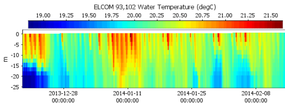
Figure 26 Simulated water temperatures during the summer (2013/2014) modelling period.
