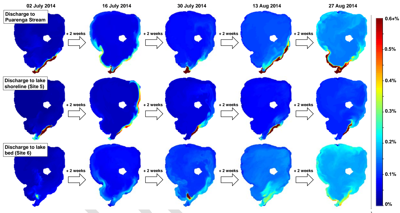
Figure 36 Comparison of simulated surface water (0–2 m) tracer concentrations for scenarios of discharge to the Puarenga Stream, Lake Rotorua shoreline (Site 5) and the lake bed (Site 6; Map 2) during winter 2014. Plots are at two-week intervals, commencing two-weeks after the simulation started.
