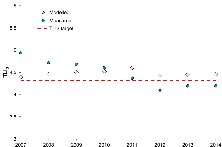
Figure 21 Comparison of modelled and measured annual TLI 3 . The dashed red line denotes the TLI 3 -adjusted target for Lake Rotorua.
