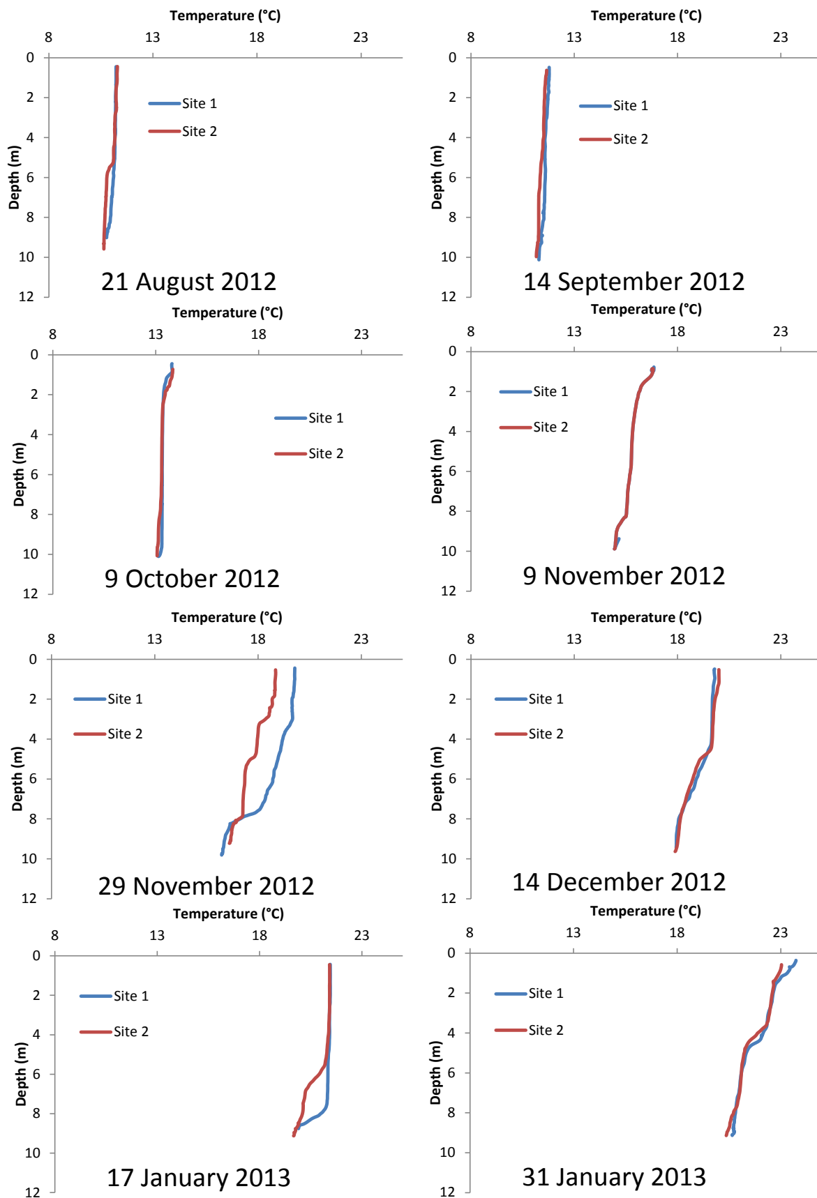
Figure 12. Comparison of CTD casts taken at Site 1 (mixing devices location) and Site 2 (c. 400 m from mixing devices). The mixing devices were active from mid-November 2012.
