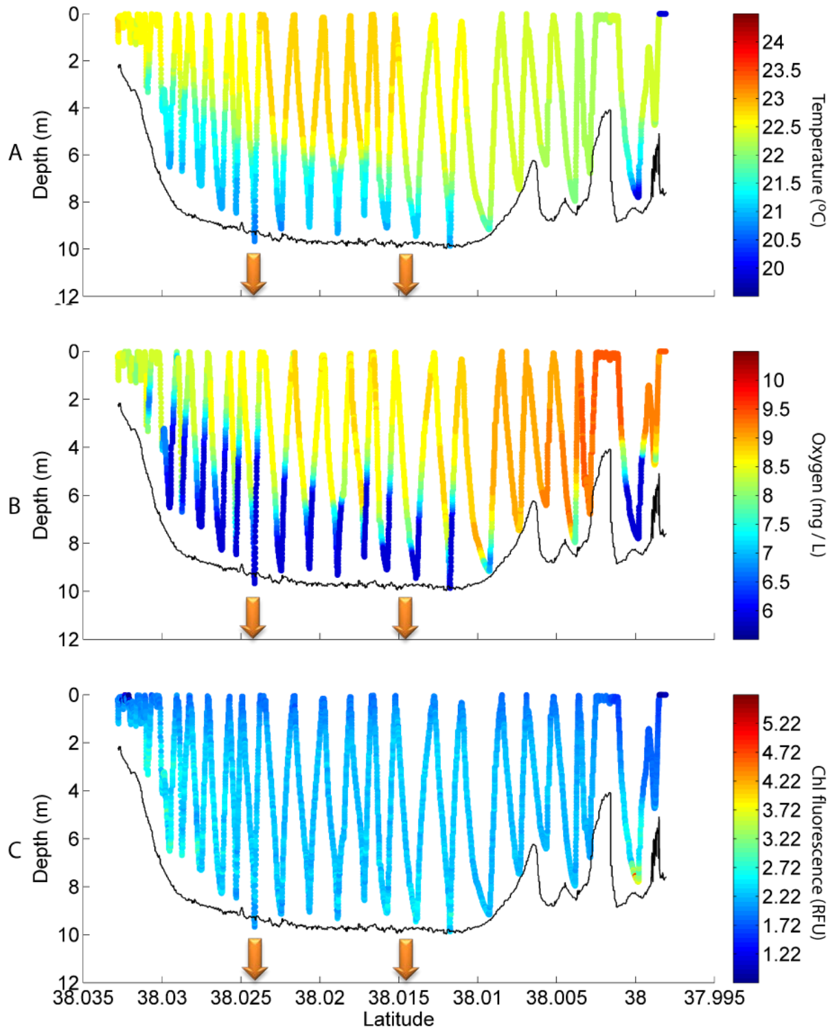
Figure 17. Cross section of Lake Rotoehu showing the undulating path of the Bio-Fish device through the water on 22 February 2013 for A) water temperature, B) dissolved oxygen concentration, and C) chlorophyll fluorescence. The lake was strongly stratified with evidence of oxygen depletion in bottom waters. Note uneven depth of stratification across the transect. Orange arrows denote the location of the mixing devices. The Bio-Fish passed within 100 m of the southern machine, and approximately 350 m from the northern machine (see Figure 2).
