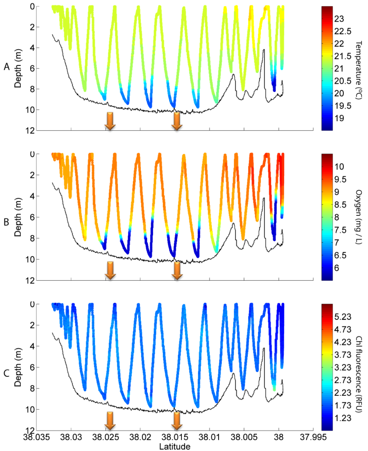
Figure 16. Cross-section of Lake Rotoehu showing the undulating path of the Bio-Fish device through the water on 17 January 2013 for A) water temperature, B) dissolved oxygen concentration, and C) chlorophyll fluorescence. Orange arrows denote the location of the mixing devices. The Bio-Fish passed within 100 m of the southern machine, and approximately 350 m from the northern machine (see Figure 2).
