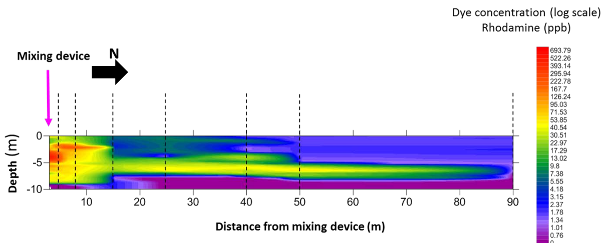
Figure 20. Contour plot of the dye plume from the mixing device on 27 February 2013 using Surfer32 by Golden Software. Vertical lines are profiling points. Extrapolation between points used triangulation with a ratio of 12:1. The contour plot is a representation of the likely dye flow path based on the available data.
