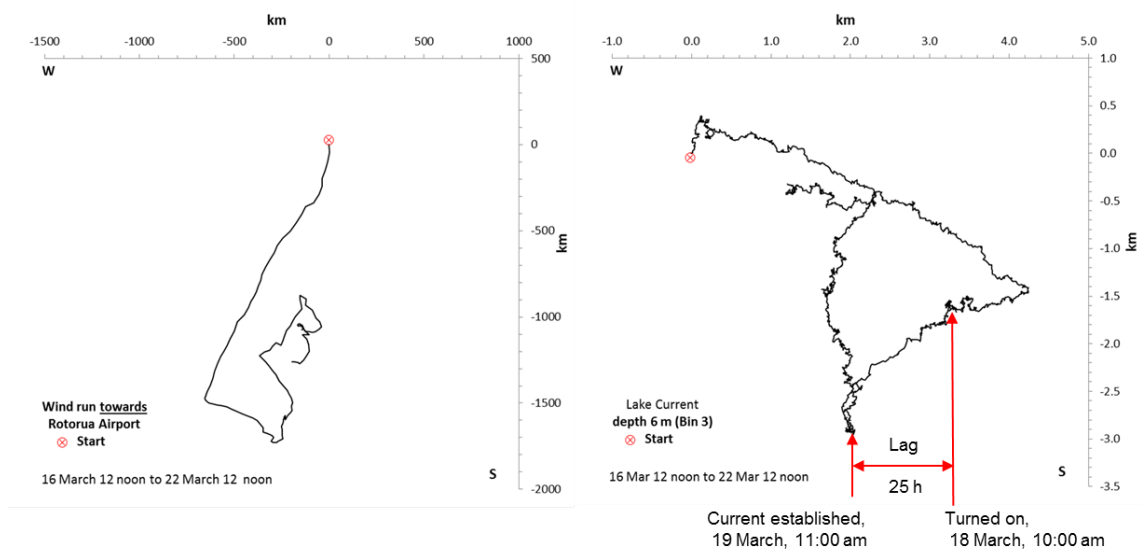
Figure 24. Estimating the time lag for the mixing device current to be established after switch on.
