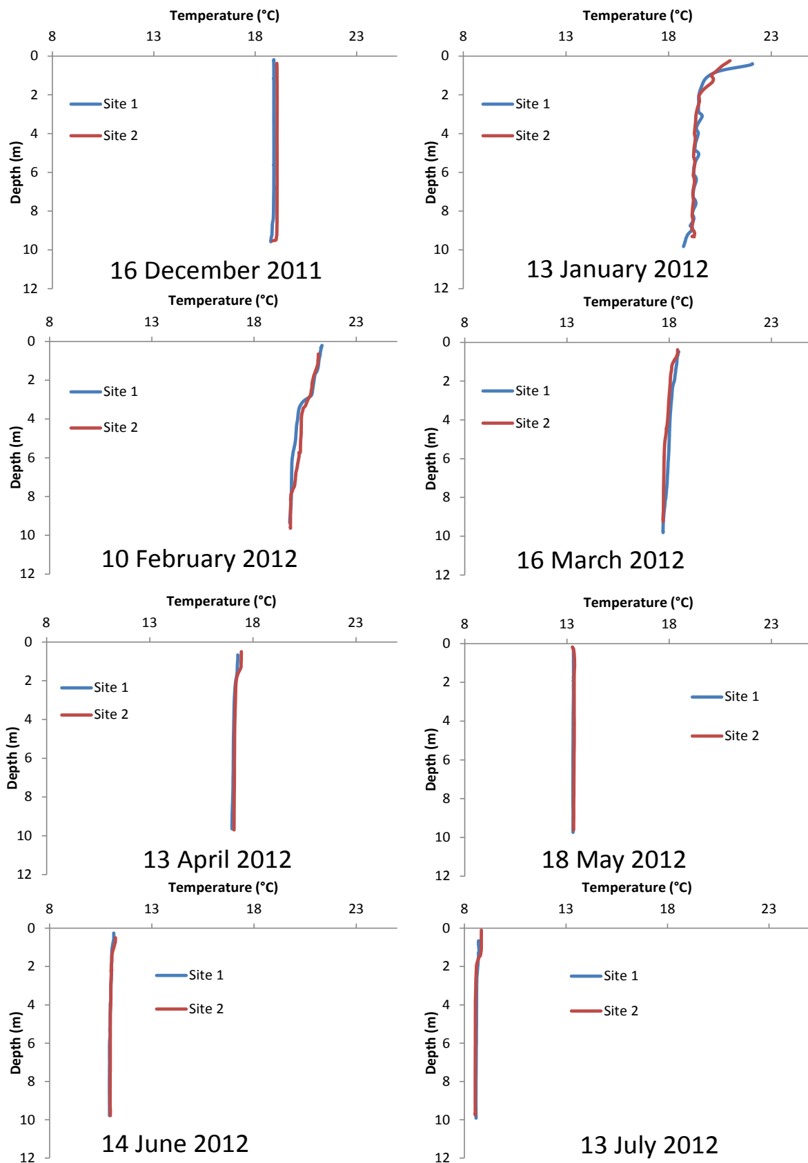
Figure 11. Comparison of CTD casts taken at Site 1 (mixing device location) and Site 2 (c. 400 m from mixing device). Casts presented are prior to installation of the mixing devices.
