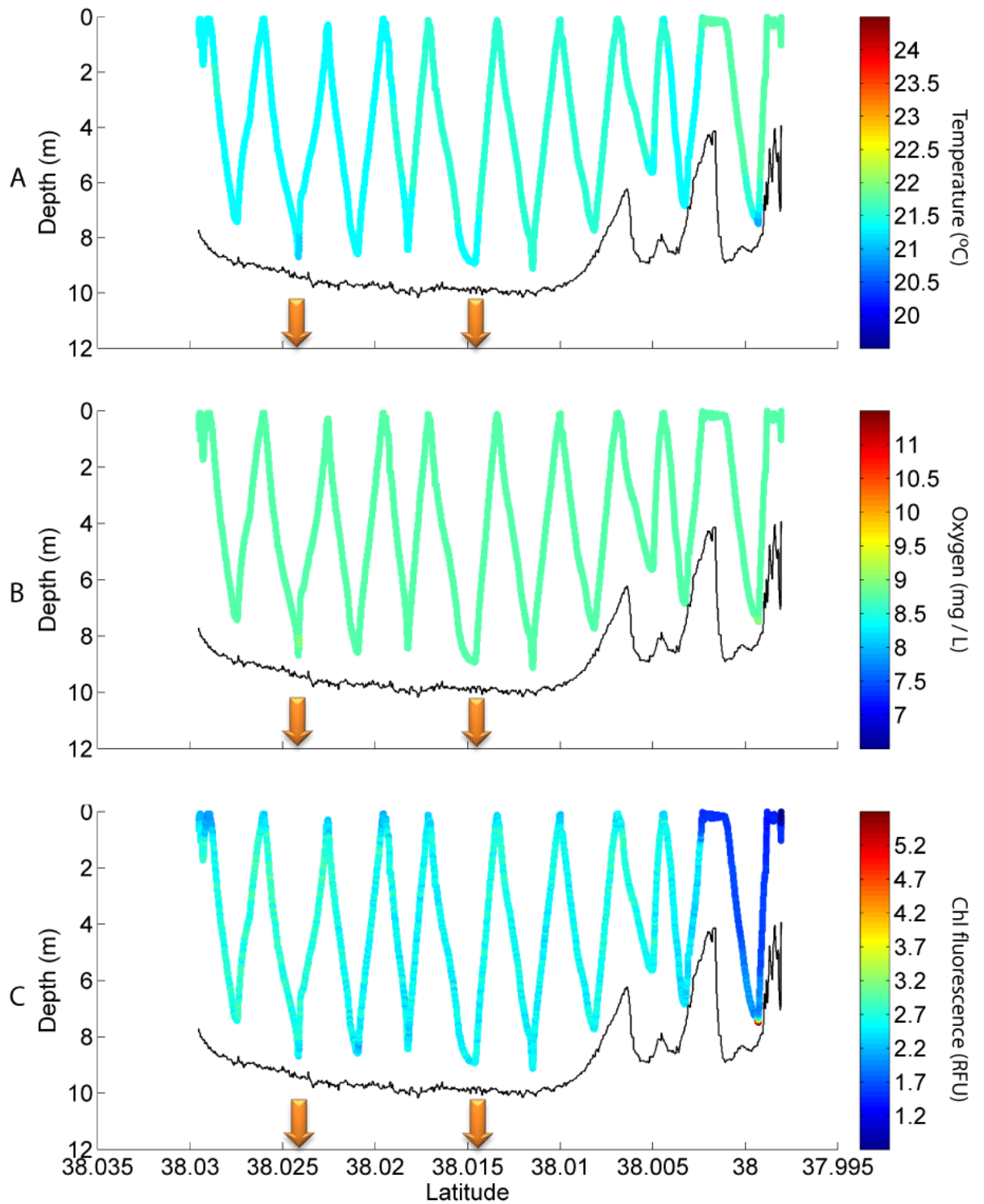
Figure 18. Cross-section of Lake Rotoehu showing the undulating path of the Bio-Fish device through the water on 01 March 2013 for A) water temperature, B) dissolved oxygen concentration and C) chlorophyll fluorescence. Orange arrows denote the location of the mixing devices. The Bio-Fish passed within 100 m of the southern machine, and approximately 350 m of the northern machine (see Figure 2). The mixing devices were turned off on this occasion, although the lake was already fully mixed on this day.
