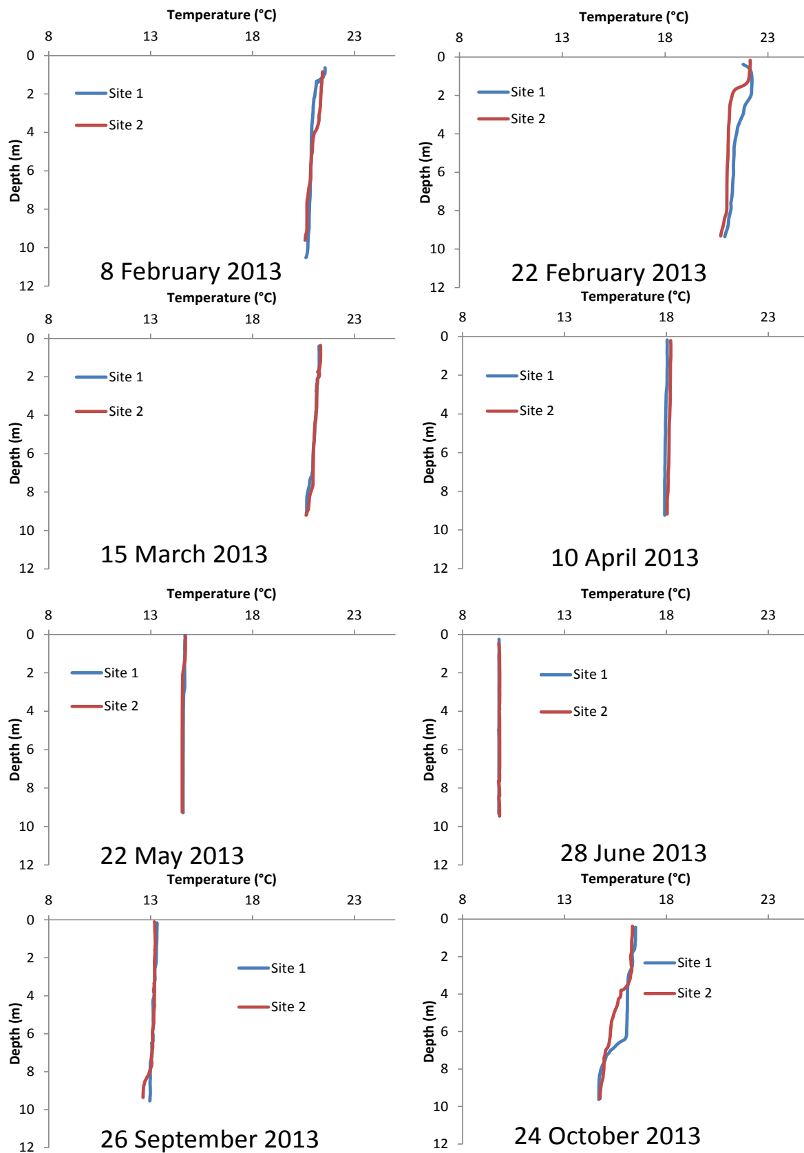
Figure 13. Comparison of CTD casts taken at Site 1 (mixing devices location) and Site 2 (c. 400 m from mixing devices). The mixing devices were not in operation on 15 March, 28 June, 26 September and 24 October 2013.
