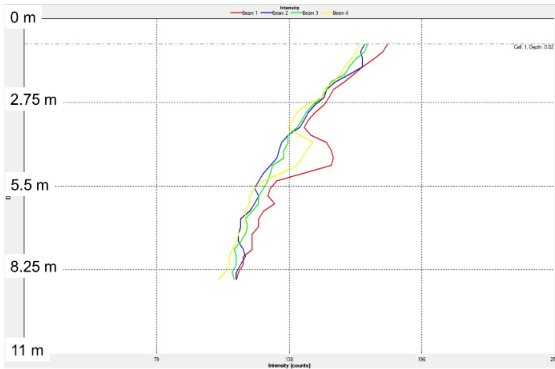
Figure 22. Example of the flow pattern from the southern mixing device through the water column depth adjacent to the western arm of the device (Figure 22, arm A) at a distance of 12 m.
