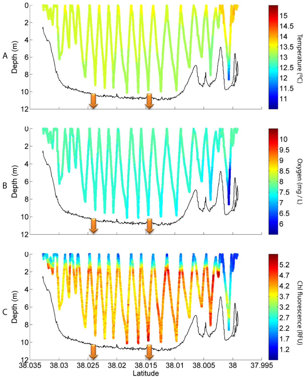
Figure 15. Cross-section of Lake Rotoehu showing the undulating path of the Bio-Fish device through the water on 9 October 2012 for A) water temperature, B) dissolved oxygen concentration, and C) chlorophyll fluorescence. Fluorescence data are reduced near the water surface, likely indicating non-photochemical quenching (bright-light inhibition of phytoplankton fluorescence response). Orange arrows denote the location of the mixing devices. The Bio-Fish passed within 100 m of the southern machine, and approximately 350 m from the northern machine (see Figure 2).
