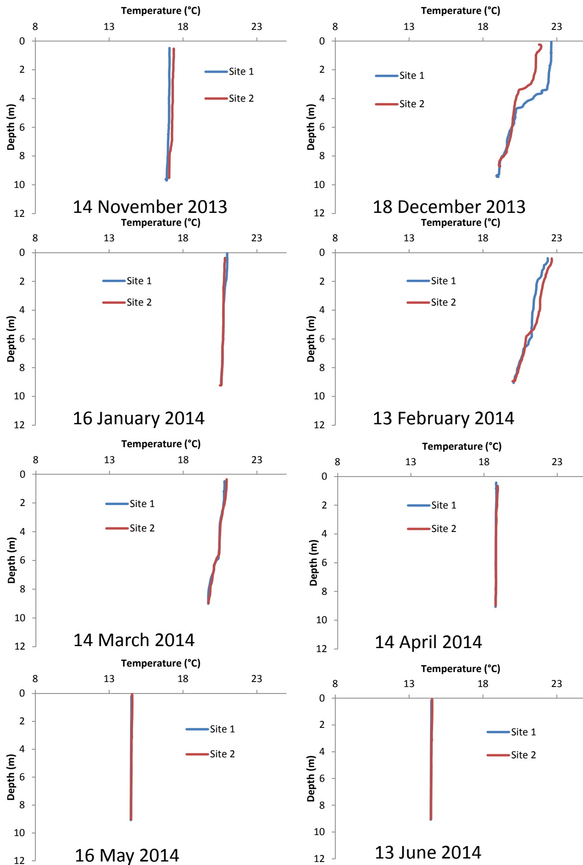
Figure 14. Comparison of CTD casts taken at Site 1 (mixing devices location) and Site 2 (c. 400 m from mixing device). Mixing devices were in operation from 14 November 2013 to 13 June 2014.
